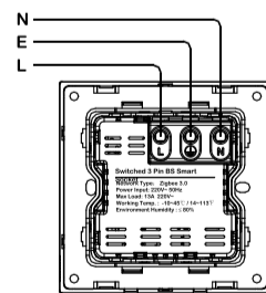
Switched 3 Pin BS Smart Socket
