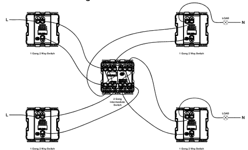
2 Gang Intermediate Switch
