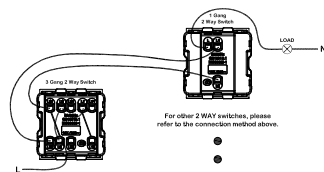
3 Gang 2 Way Switch
