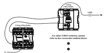
4 Gang 2 Way Switch
